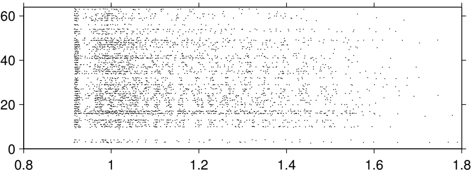
activity evoked by ChR2 during 40uM CNQX application
